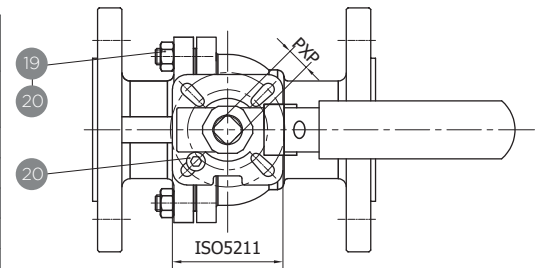
Actuator connection dimensions (OB1) and (OB2) according to ISO 5211
