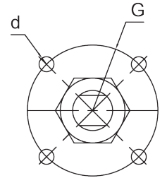
ACTUATOR CONNECTION
